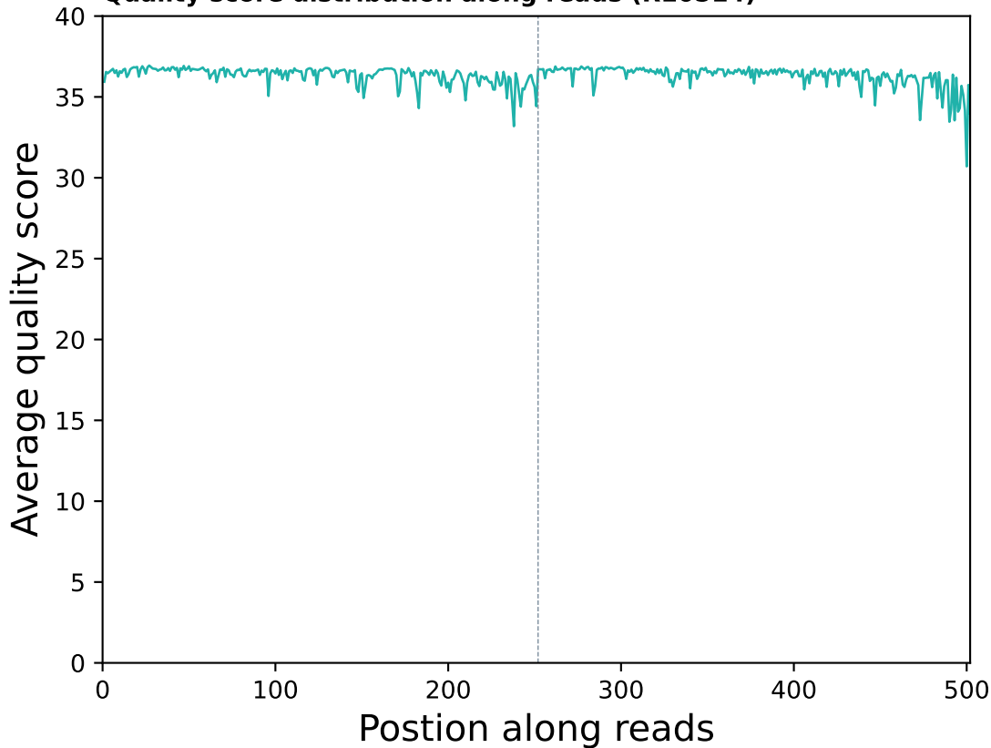
Quality score distribution along reads (R10514)
